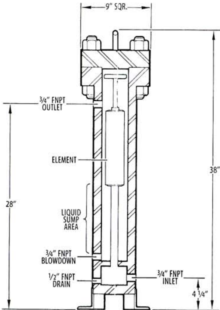
Replaceable Coalescing Element
